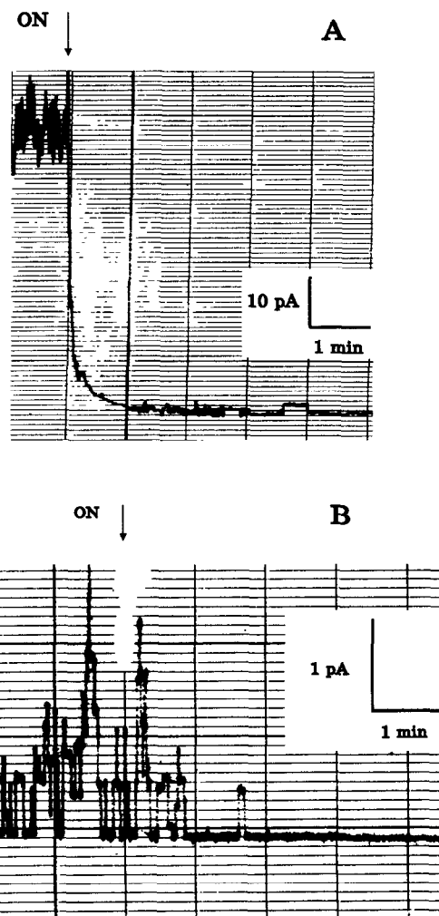
Fig. 2. The effect of visible light irradiation ( 30 \text{ mW/cm}^2 ) on gramicidin-induced BLM conductance in the presence of phthalocyanine. (A) 4 \cdot 10^{-12} \text{ M} gramicidin, 1 \mu\text{M AlPcS}_3 . (B) 2 \cdot 10^{-13} \text{ M} gramicidin, 10 \mu\text{M AlPcS}_4 .
