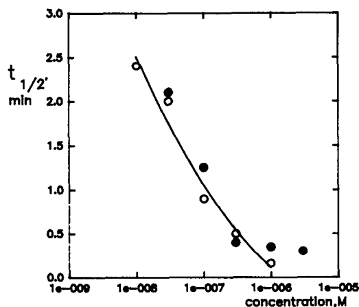
Fig. 3. The dependence of the time to produce a 50% decrease in the gramicidin-induced conductance ( t_{1/2} ) on the concentration of phthalocyanine. The incident power density of the light produced by the He-Ne laser is 30 mW/cm 2 . (○) AlPcS 3 ; (●) AlPcS 4 .
